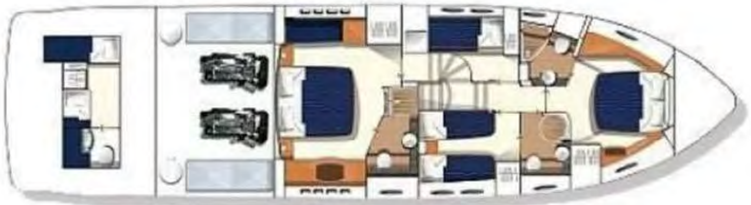
Lower accommodation layout
